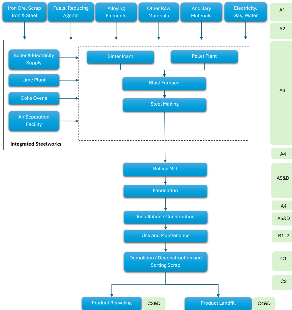
Overview of Product System for Carbon Steel Slab
